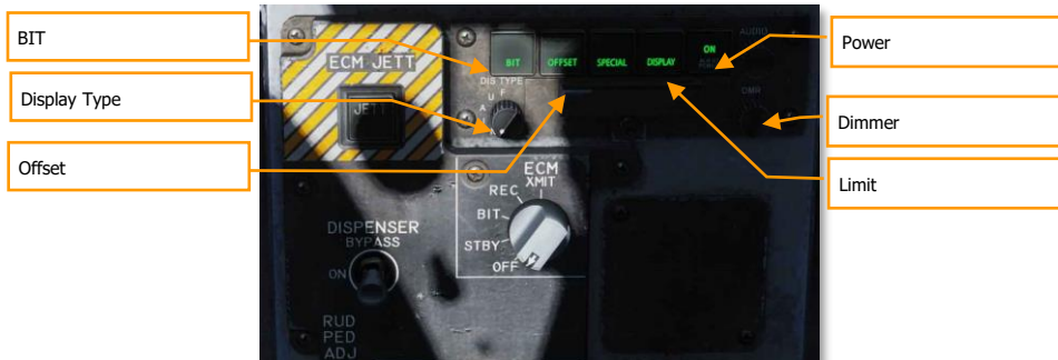
Figure 234. Control Indicator Panel
