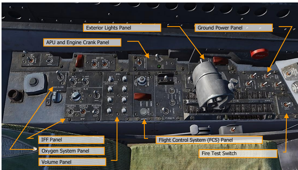
Figure 15. Left Console
