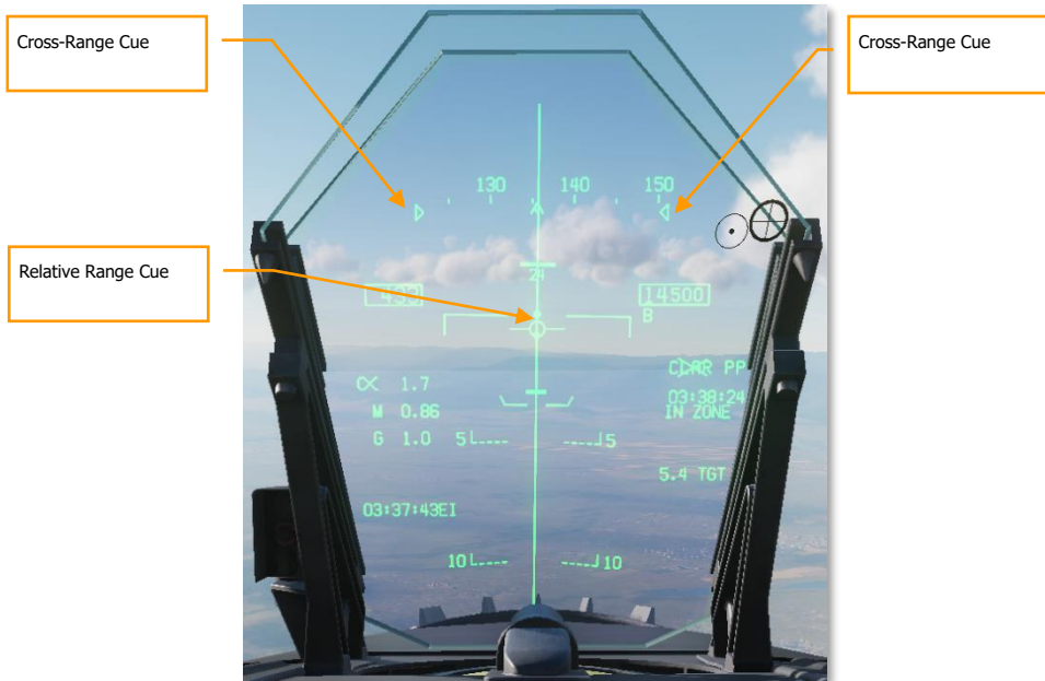
Figure 177. Paveway III HUD, In LAR
