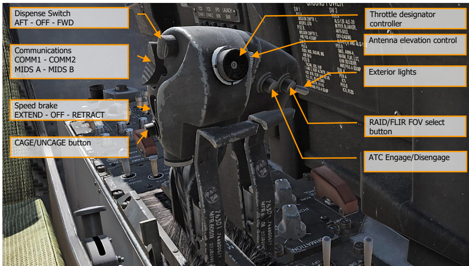
Figure 21. Throttles
