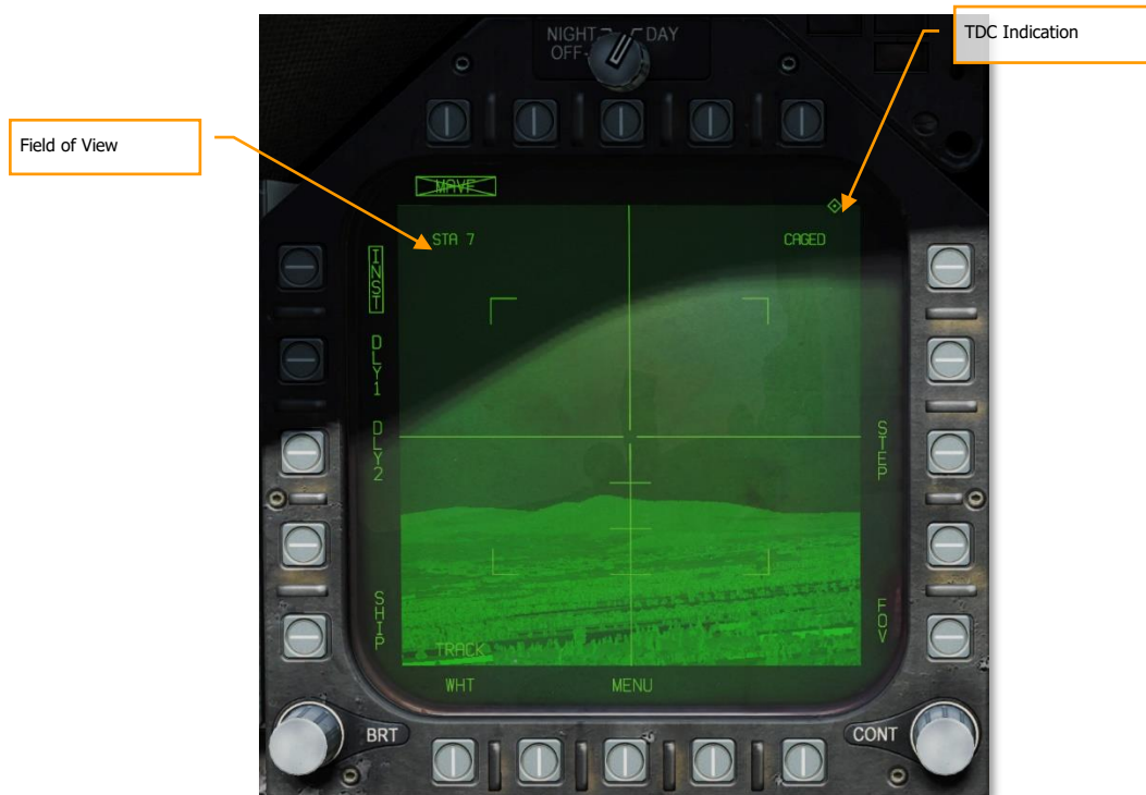
Figure 196. AGM-65F Video
